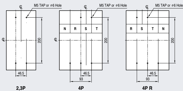
Perforacion del panel
